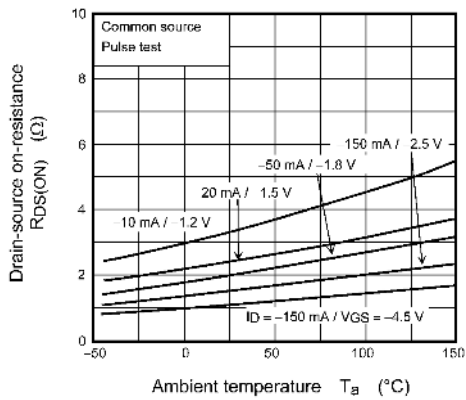
Fig. 7.5 R_{DS(ON)} - T_a
