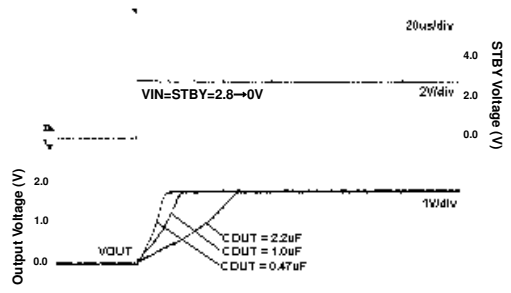
Fig 25. Start Up Time (VIN=STBY) Iout=200mA
