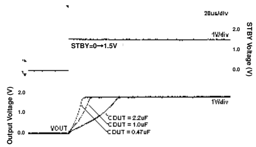
Fig 23. Start Up Time Iout=200mA
