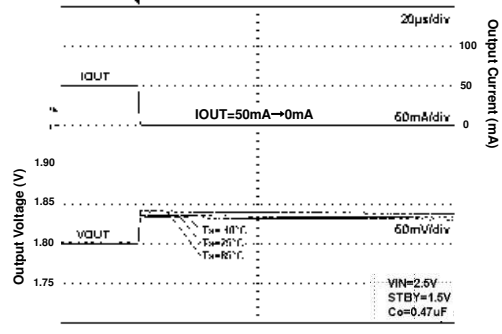
Fig 15. Load Response
