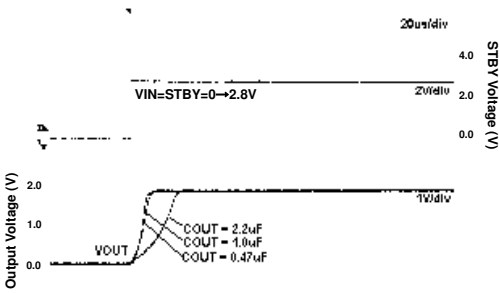
Fig 24. Start Up Time (VIN=STBY) Iout=0mA Iout=0mA
