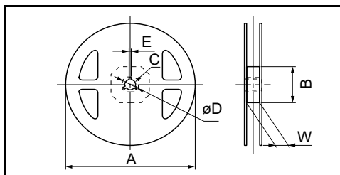
Standard Reel Dimensions
