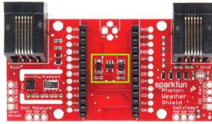
On-board 3.3V regulator and accompanying circuitry.
