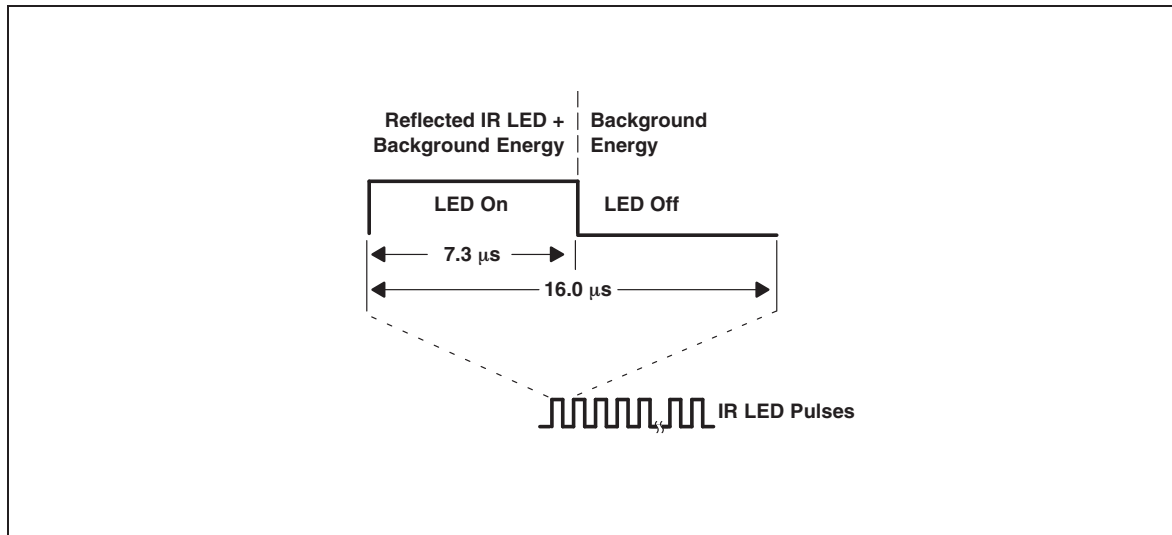
Figure 19: Proximity LED Current Driver Waveform
