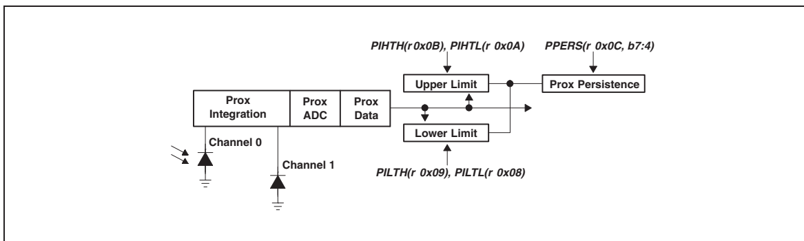
Figure 20: Programmable Interrupt
