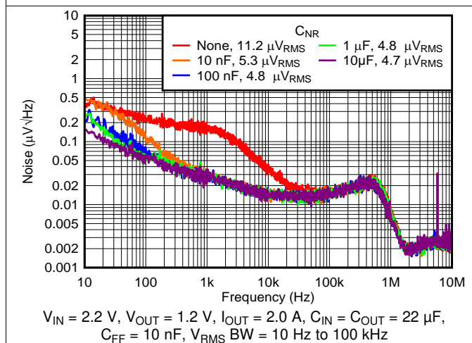
Figure 9. Spectral Noise Density vs Frequency and C_{NR/SS}
