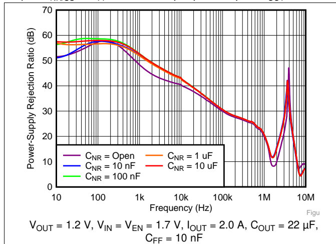
Figure 7. PSRR vs Frequency and C_{NR/SS}
