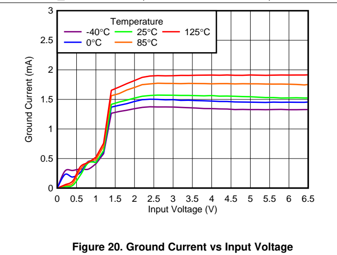
Figure 20. Ground Current vs Input Voltage
