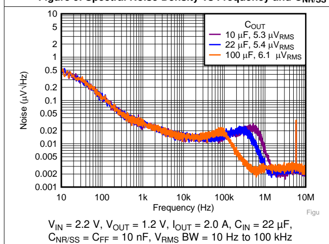
Figure 11. Spectral Noise Density vs Frequency and C_{OUT}
