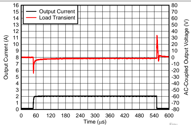
Figure 30. Load Transient Response ( V_{OUT} = 5.0\text{ V} ) V_{IN} = 5.5\text{ V} , I_{OUT} = 100\text{ mA to } 2\text{ A to } 100\text{ mA at } 1\text{ A}/\mu\text{s} , C_{OUT} = 22\ \mu\text{F} , V_{PG} = V_{OUT}
