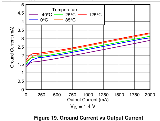
Figure 19. Ground Current vs Output Current
