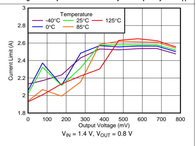
Figure 12. Current Limit Foldback
