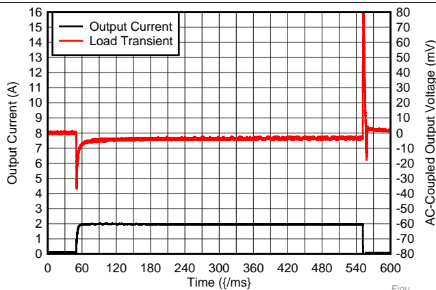
Figure 29. Load Transient Response ( V_{OUT} = 1.2\text{ V} ) V_{IN} = 1.5\text{ V} , I_{OUT} = 100\text{ mA to } 2\text{ A to } 100\text{ mA at } 1\text{ A}/\mu\text{s} , C_{OUT} = 22\ \mu\text{F} , V_{PG} = V_{OUT}
