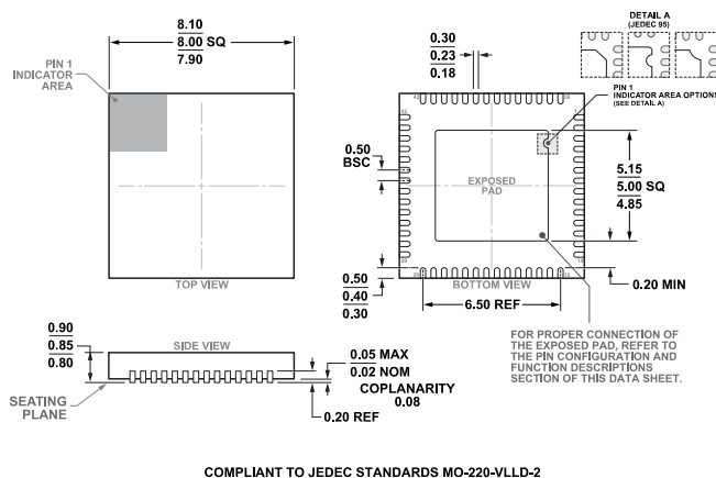
Figure 53. 56-Lead Lead Frame Chip Scale Package [LFCSP] 8 mm × 8 mm Body and 0.85 mm Package Height (CP-56-21) Dimensions shown in millimeters
