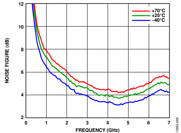
Figure 8. Noise Figure vs. Frequency for Various Temperatures
