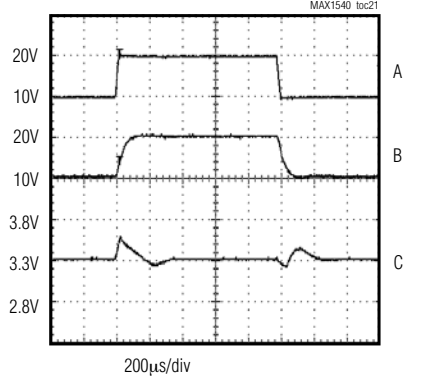
A. INPUT ( V_{IN} ), 10V/div B. LDoin (10V TO 20V), 10V/div C. LDooout (3.3V), 500mV/div 20mA LOAD
