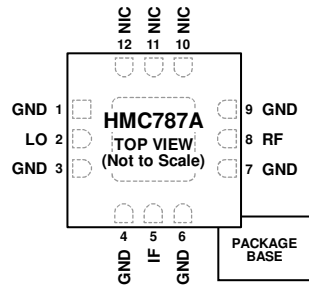
Figure 2. Pin Configuration
