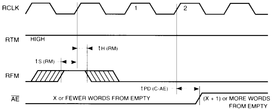
FIGURE 15. \overline{\text{AE}} MAXIMUM LATENCY WHEN RETRANSMIT INCREASES THE NUMBER OF STORED WORDS ABOVE X
