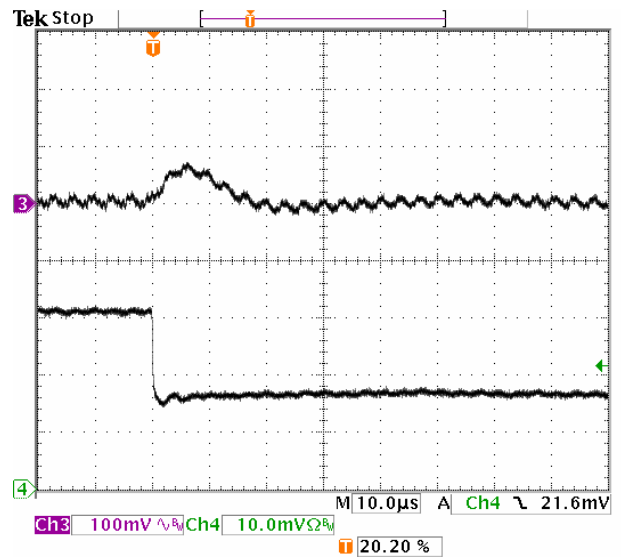
Fig-1.5V-7: Output voltage response for V_{out}=1.5V to positive load current step-change from 3A to 1.5A with slew rate of -5A/\mu s at V_{in}=5.0V . C_o=47\mu F \times 2 ceramic.
