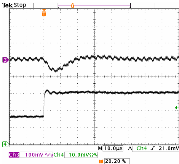
Fig-1.5V-6: Output voltage response for V_{out}=1.5V to positive load current step-change from 1.5A to 3A with slew rate of 5A/\mu s at V_{in}=5.0V . C_o=47\mu F \times 2 ceramic.
