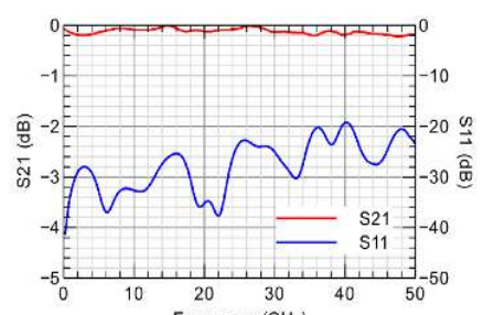
Fig.3: 5.6 nF/0201M UBSC @ BV30 measurement results (S-parameters in transmission mode) Modelithics FREE S-Parameters-Based Linear Simulation Models for ADS: http://www.modelithics.com
