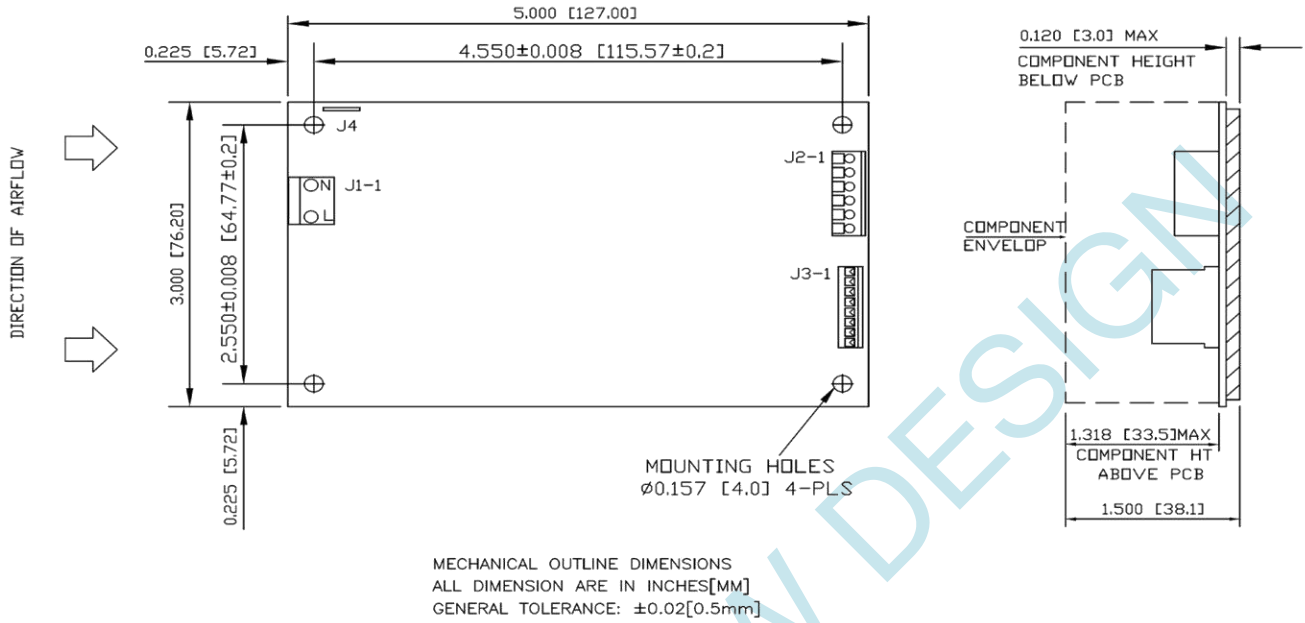
Figure 2. Mechanical Drawing
