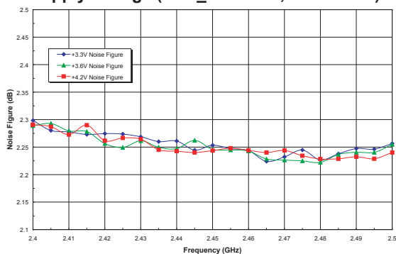
Figure 22: Receive Path Noise Figure Across Supply Voltage ( V_{LNA\_EN}=+3.3\text{ V} , T_A = +25^\circ\text{C} )
