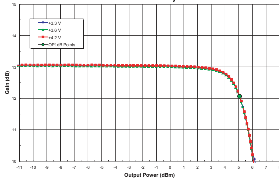
Figure 24: Receive Path Output P1dB Across Supply Voltage (Freq =2.45 GHz, V_{LNA\_EN}=+3.3\text{ V} , T_A = +25^\circ\text{C} )
