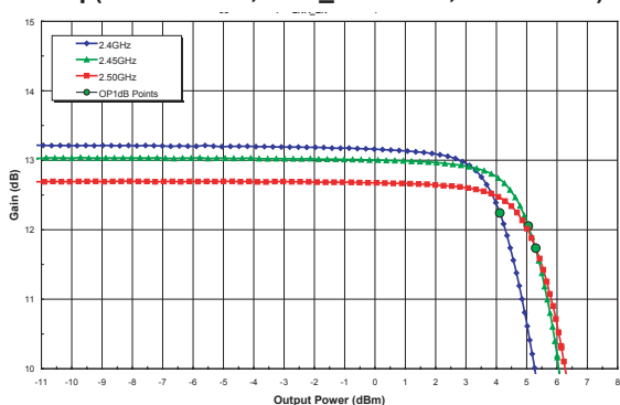
Figure 23: Receive Path Output P1dB Across Freq ( V_{CC} = +3.6\text{ V} , V_{LNA\_EN}=+3.3\text{ V} , T_A = +25^\circ\text{C} )
