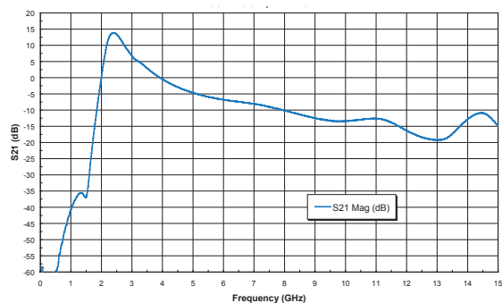
Figure 25: Rx Path S-Parameters S21 Response ( V_{CC} = +3.6\text{ V} , T_A = +25^\circ\text{C} )
