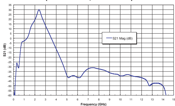
Figure 20: Tx Path S-Parameters S21 Response ( V_{CC} = +3.6\text{ V} , T_A = +25^\circ\text{C} )
