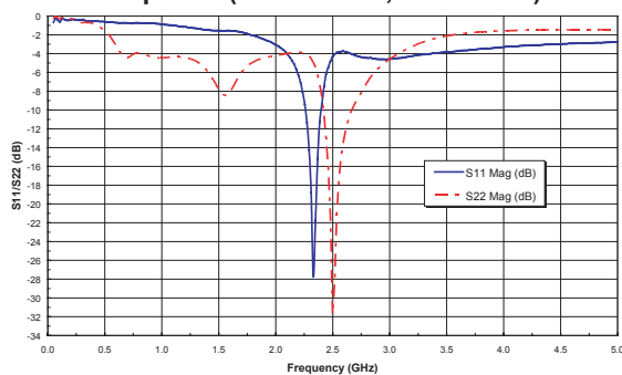
Figure 21: Tx Path S-Parameters S11 & S22 Response ( V_{CC} = +3.6\text{ V} , T_A = +25^\circ\text{C} )
