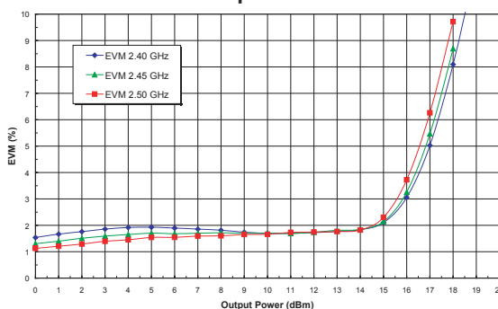
Figure 5: Tx Path EVM vs. Output Power Across Freq ( V_{CC} = +3.6\text{ V} , T_A = +25^\circ\text{C} ) 802.11g 54 Mbps OFDM
