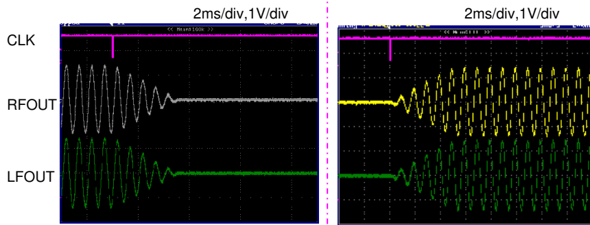
Soft mute ON (Mute setting Time ;5.12ms)
