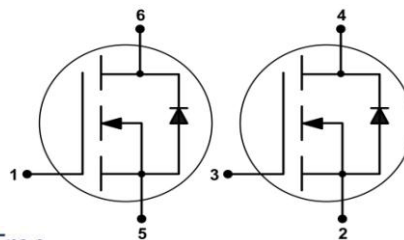
PG-TSOP6
