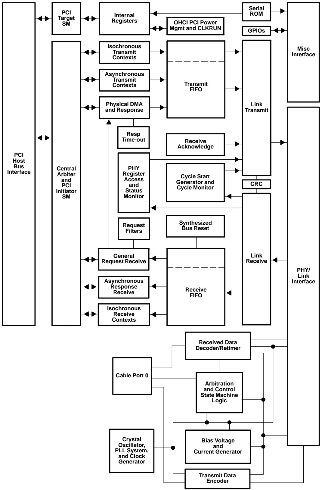
Figure 3–1. TSB43AB21 Block Diagram
