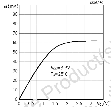
Figure 5. Output current vs output low voltage for driver
