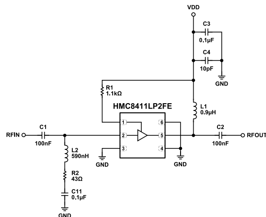
Figure 70. Typical Application Circuit
