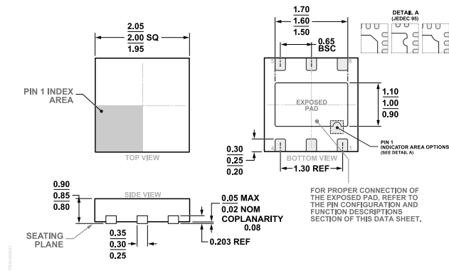
Figure 73. 6-Lead Lead Frame Chip Scale Package [LFCSP] 2 mm x 2 mm Body and 0.85 mm Package Height (CP-6-12) Dimensions shown in millimeters
