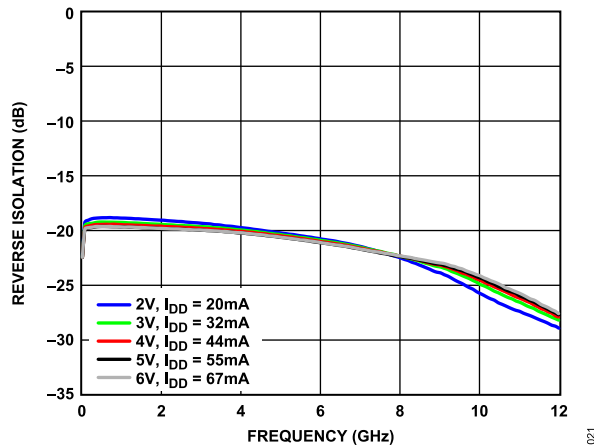
Figure 21. Reverse Isolation vs. Frequency for Various Supply Voltages and I_{DQ} , R_{BIAS} = 1.1\text{ k}\Omega
