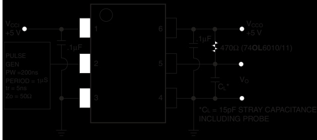
Figure 15. Switching Time Test Circuit
