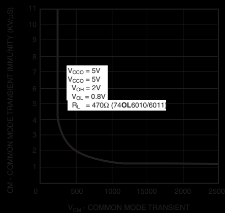
Figure 10. Common Mode Rejection vs. Common Mode Voltage
