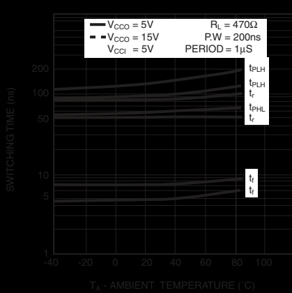
Figure 9. 74OL6010/11 Switching Times vs. Ambient Temperature
