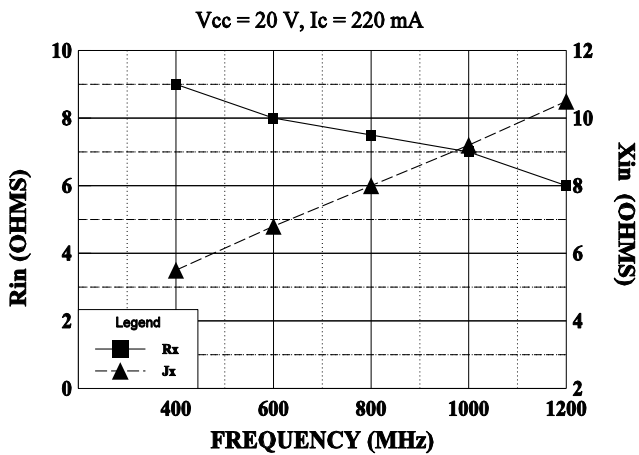
SERIES INPUT IMPEDANCE vs FREQUENCY
