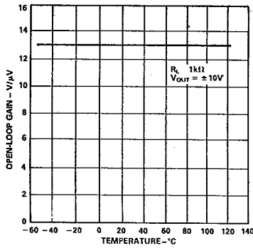
Figure 10. Open-Loop Gain vs. Temperature
