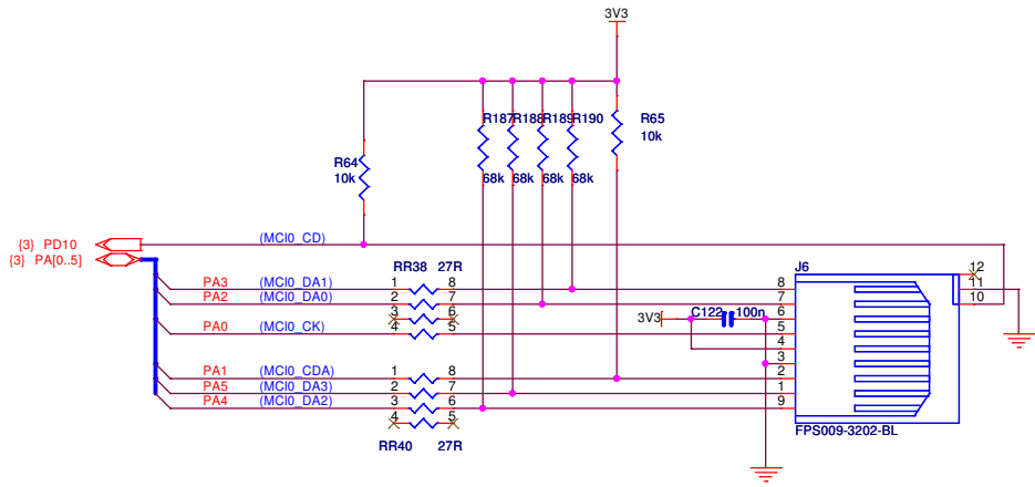
SD/MMC CARD INTERFACE - MC10
