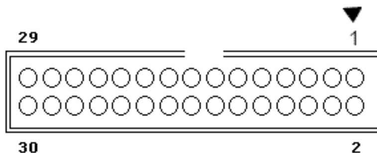
Figure 6-11. ISI Connector J17
