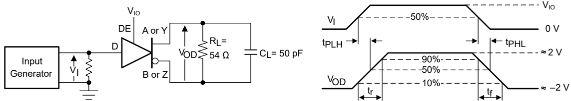
Figure 7-3. Measurement of Driver Differential Output Rise and Fall Times and Propagation Delays
