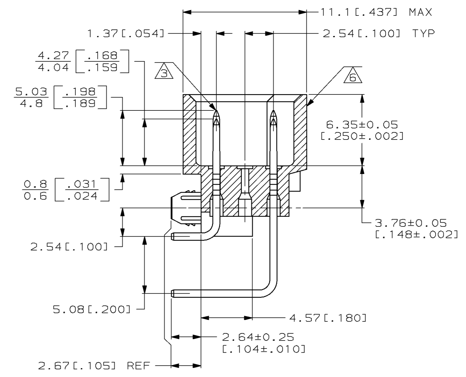
SECTION Z-Z
