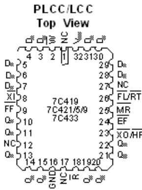
Figure 1. 32-Pin PLCC/LCC
