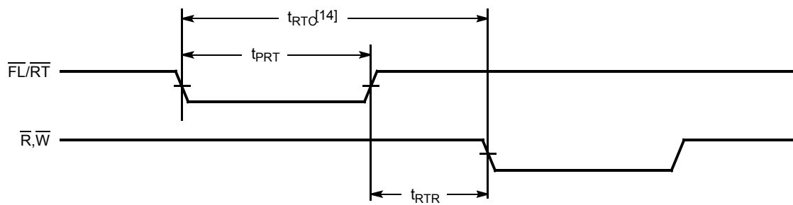
Figure 9. Retransmit [13]
