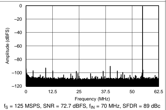
Figure 37. FFT for 70-MHz Input Signal, Dither Off
