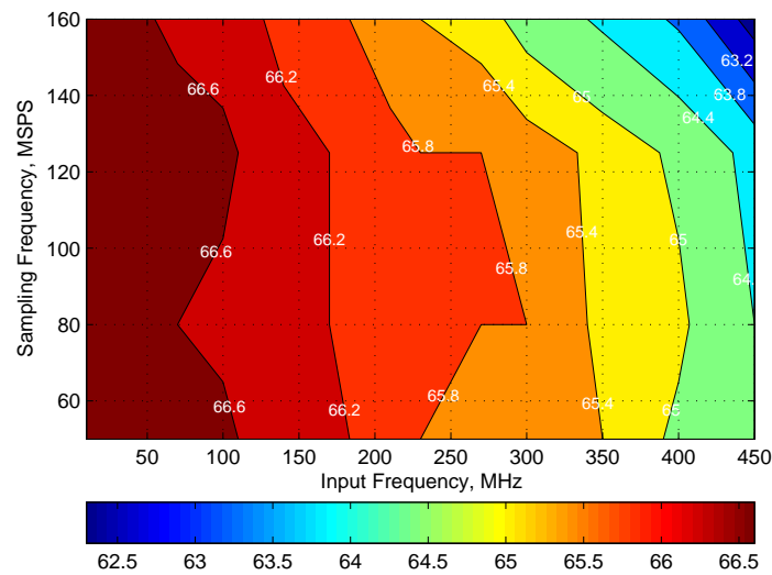
Figure 142. Signal-to-Noise Ratio (SNR) for 6-dB Gain
