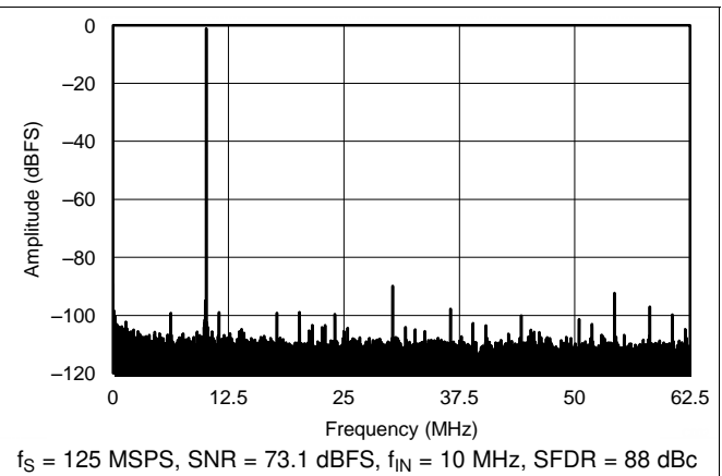
Figure 35. FFT for 10-MHz Input Signal, Dither Off
