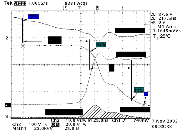
Figure 19, Turn-on Switching Waveforms and Definitions
