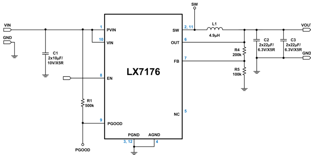
Figure 2. Typical Application with 1.8V VOUT
