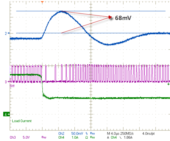
CH2: VOUT, CH3: SW, CH4: Load Current Figure 11. VOUT = 1.8V, L = 4.9µH
