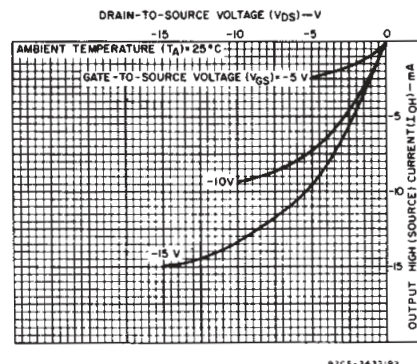
Fig. 11 - Minimum output high (source) current characteristics.
