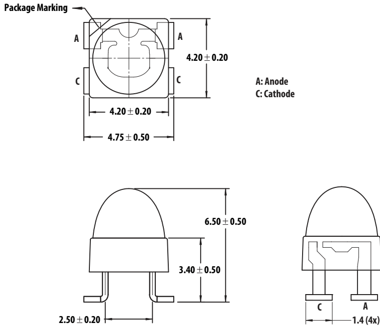
Figure 1: Package Dimensions
