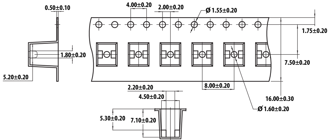
Figure 17: Carrier Tape Dimension
