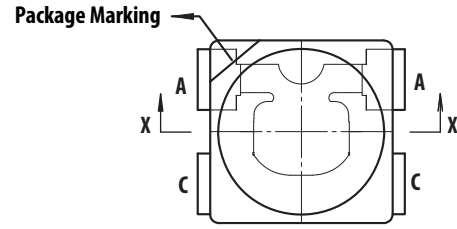
Figure 13: Component Axis for Radiation Pattern
