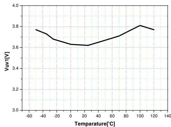
Figure 24. Output Voltage with UVLO Activated 1
