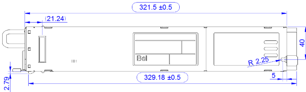
Figure 25. Top View
