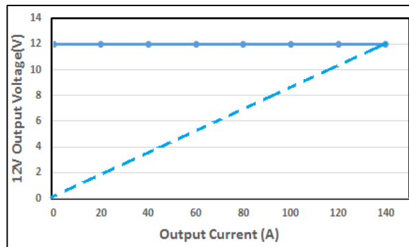
Figure 6.1 Current Limitation on V_1 ( V_i = 230\text{ VAC} )
