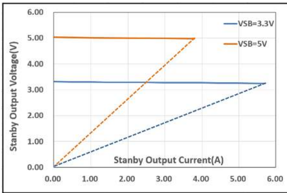
Figure 7. Current Limitation and Temperature Derating on 3.3 / 5 V SB
