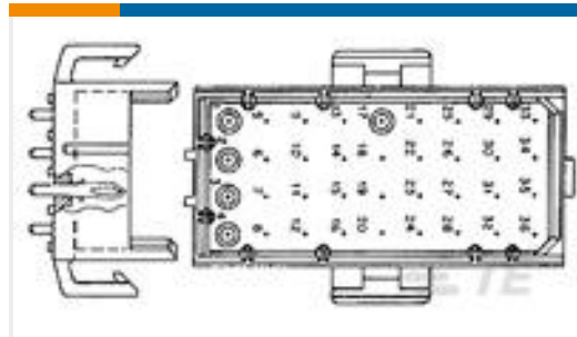
TE Part #2-640499-4 04P MR HDR ASSY VO LF
