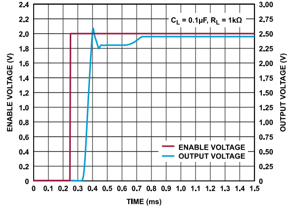
Figure 36. ADR3625 Start-Up Response (Enable)
