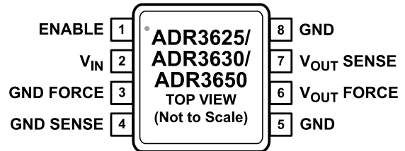
Figure 1. 8-Lead MSOP Pin Configuration
