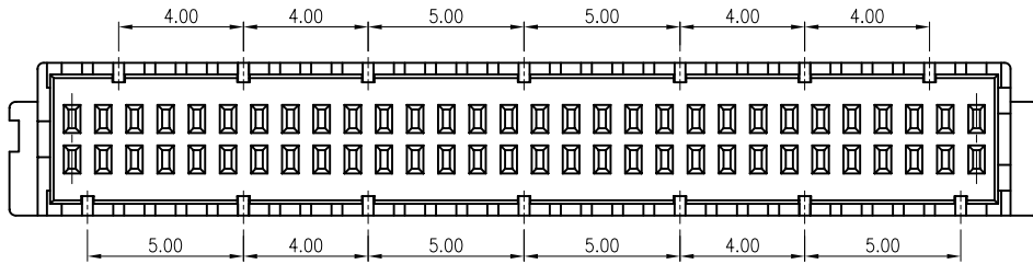
60 PIN
