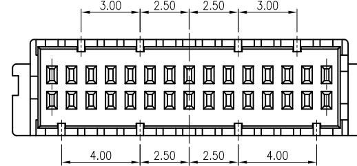
30 PIN
