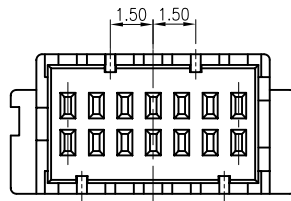
14 PIN
