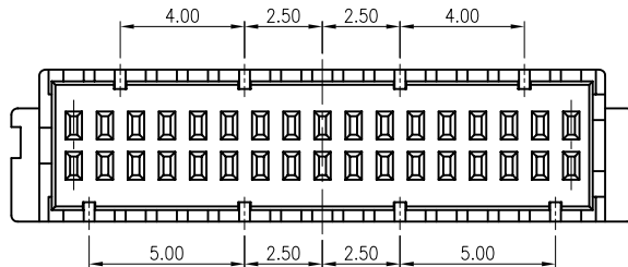
34 PIN
