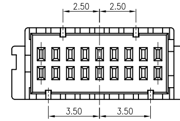
18 PIN
