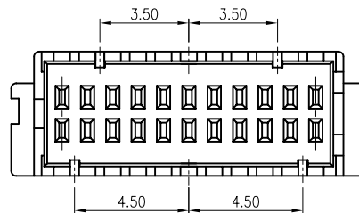
22 PIN
