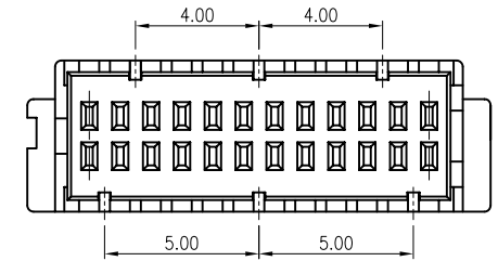
24 PIN
