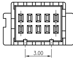
10 PIN
