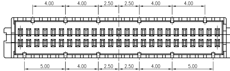
50 PIN
