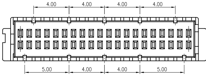
40 PIN
