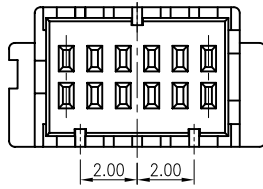
12 PIN
