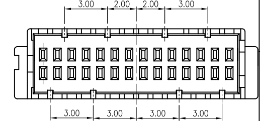
28 PIN
