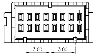
16 PIN
