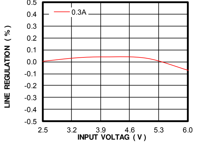
Line Regulation
