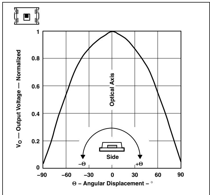
Figure 16: Normalized Output Voltage vs. Angular Displacement - T PKG
