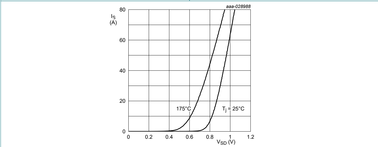
Fig. 16. Source-drain (diode forward) current as a function of source-drain (diode forward) voltage; typical values
