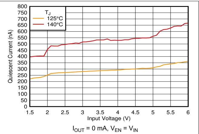
Figure 6-2. I_Q vs V_{IN} and Temperature
