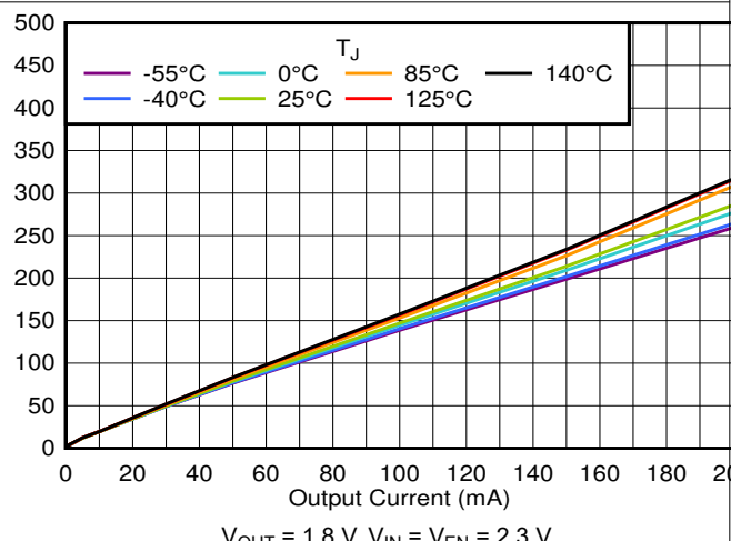
Figure 6-4. I_Q vs I_{OUT} and Temperature Up to 200 mA
