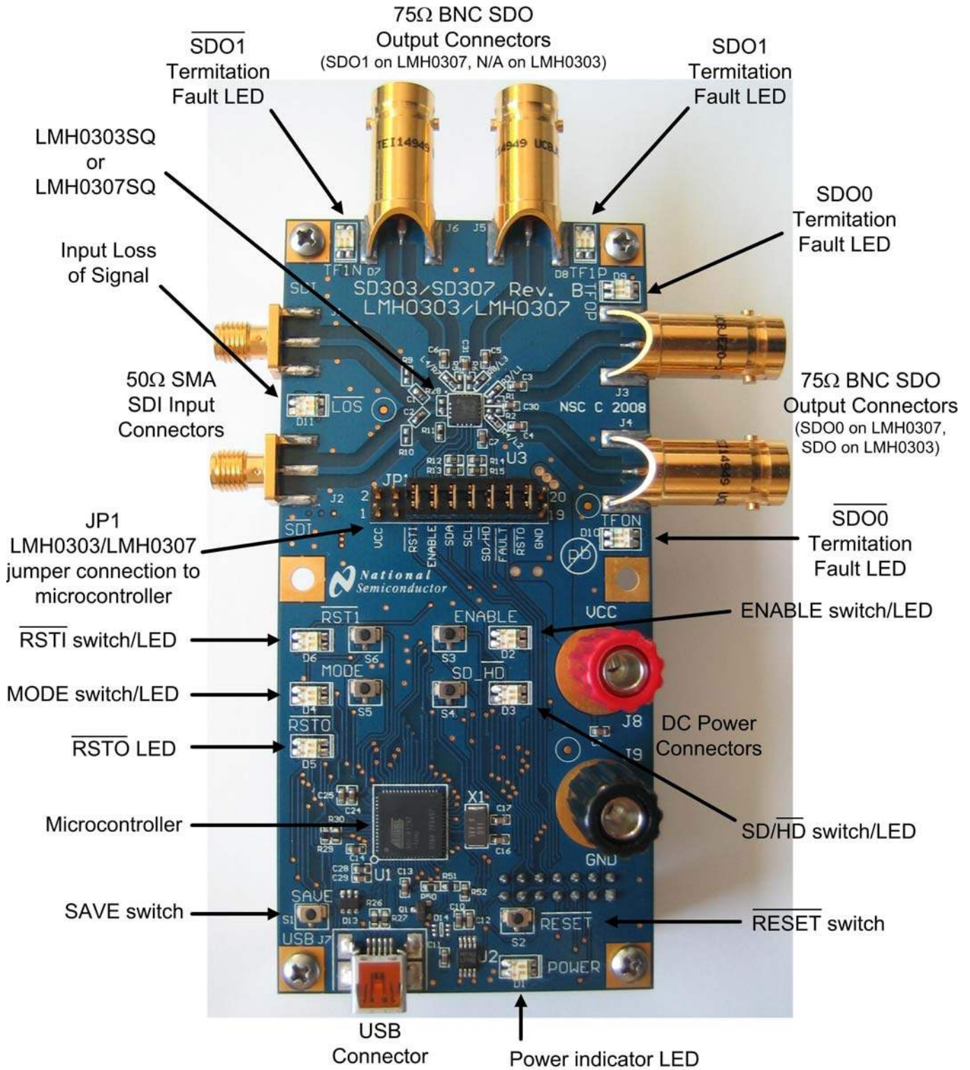
Figure 1. SD303/SD307 Evaluation Board
