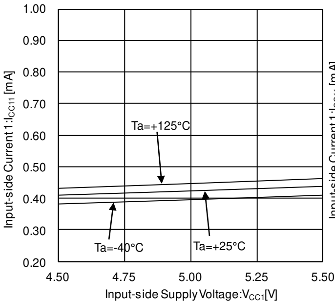
Figure 8. Input-side Circuit Current 1 vs Input-side Supply Voltage
