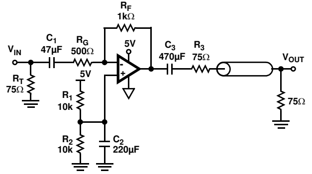
FIGURE 35. SINGLE SUPPLY INVERTING VIDEO LINE DRIVER
