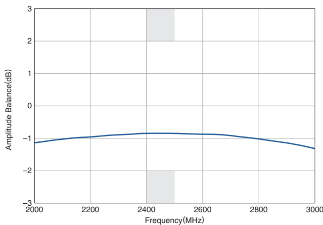
AMPLITUDE BALANCE
