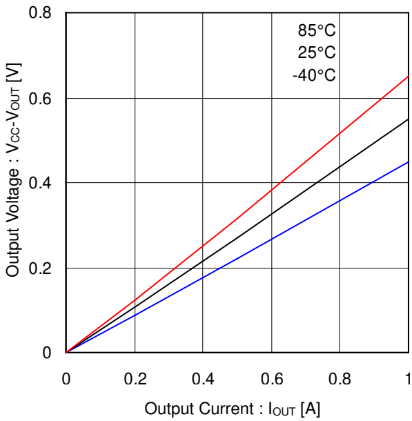
Figure 19. Output High Voltage vs Output Current (BD6211)
