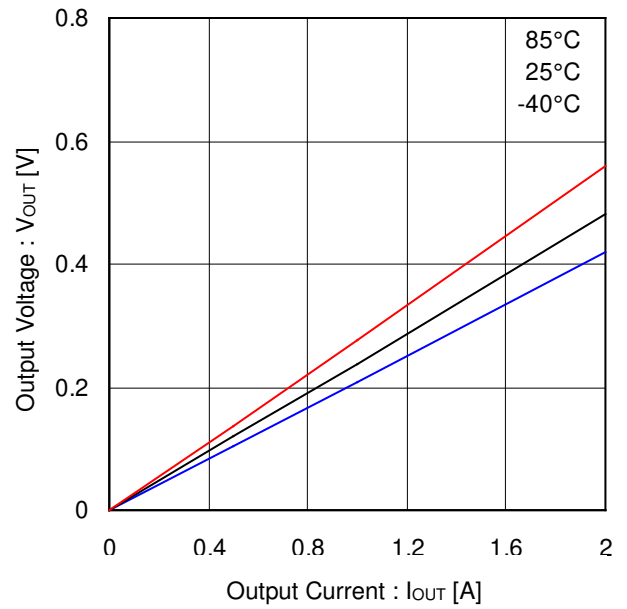
Figure 26. Output Low Voltage vs Output Current (BD6212)
