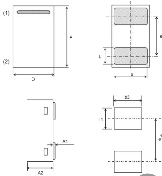
DFN1608-2, (KMD2)
