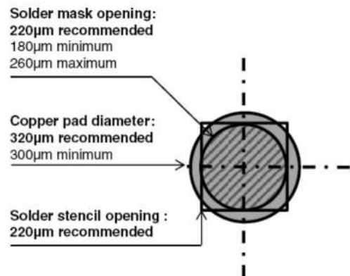
Figure 13. Footprint - solder mask defined
