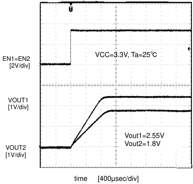
Figure.15 Soft start waveform ( I_o=0\text{mA} )
