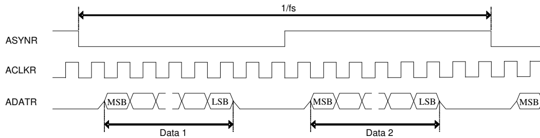
FIGURE 24. ACLKMASTER=0, RM_SYNC=0
