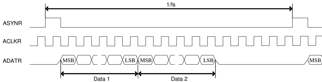
FIGURE 25. ACLKMASTER=0, RM_SYNC=1
